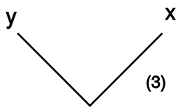
k / Two vectors, \mathbf{P} and \mathbf{Q} , to which we apply the same operation in two different frames of reference, 2 and 3.
